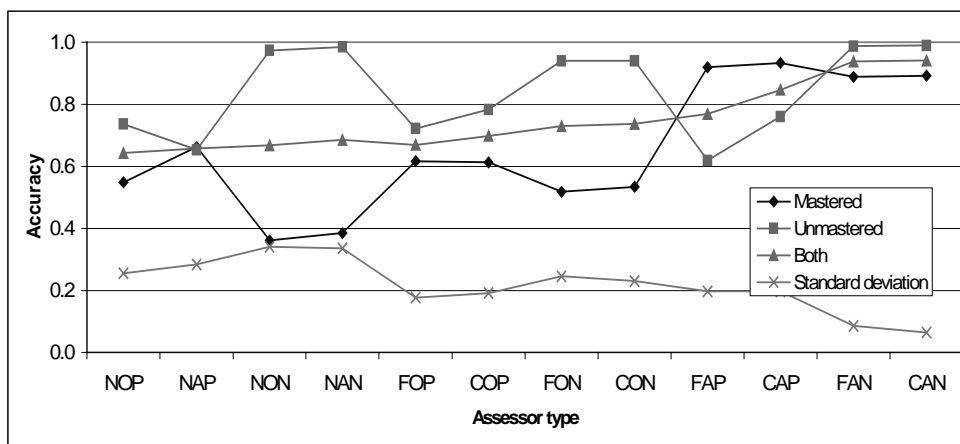
Figure 9. Average Accuracy
